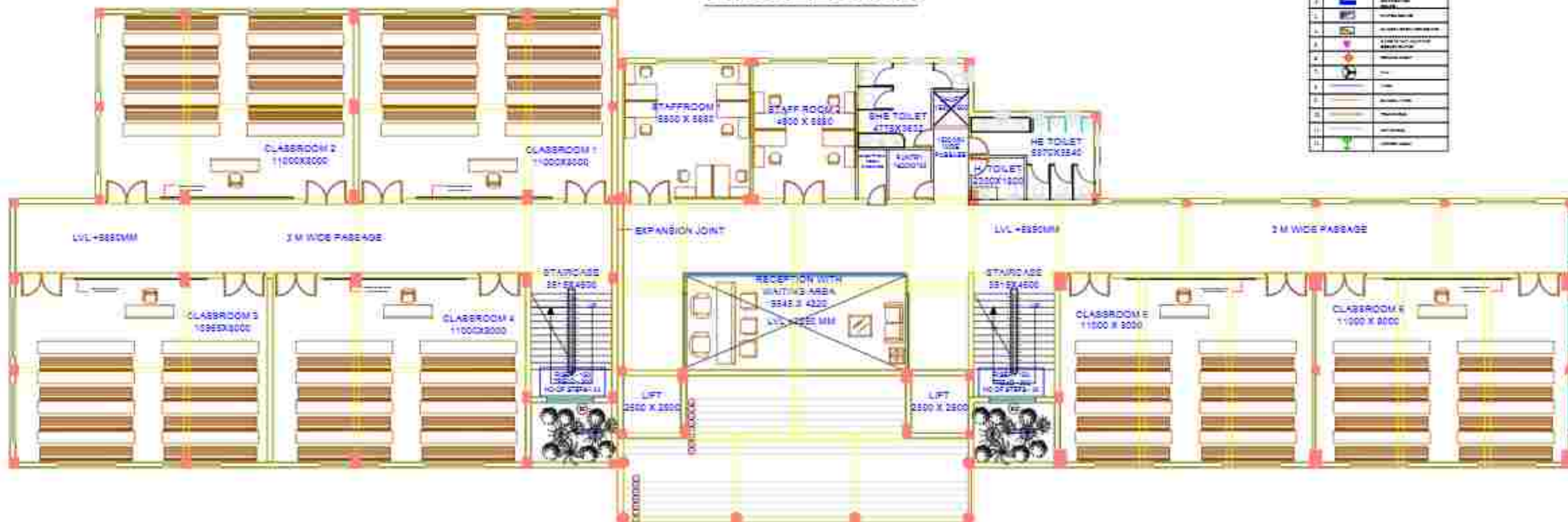
FIRST FLOOR
